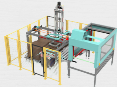
Gantry Palletizer
